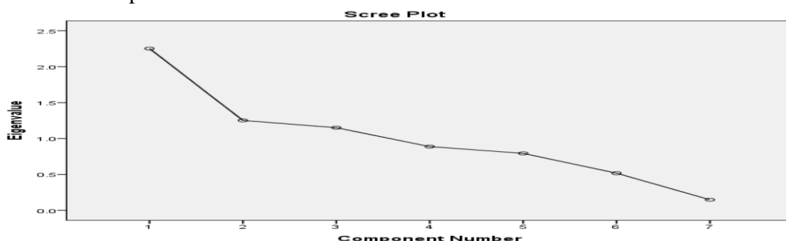
Fig 2.Component Number Test Scree Plot
