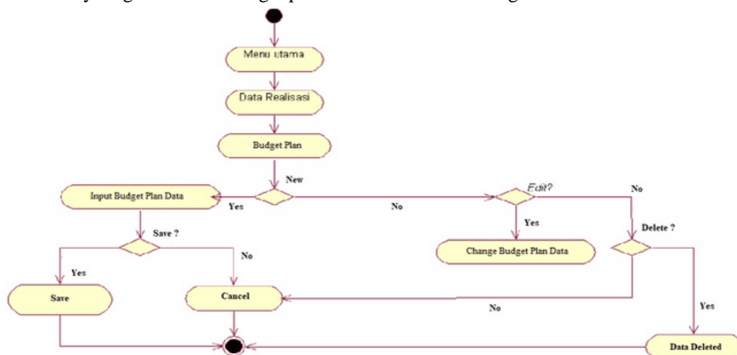
Fig 11. Activity Diagram Cost Budget Plan (RAB)
