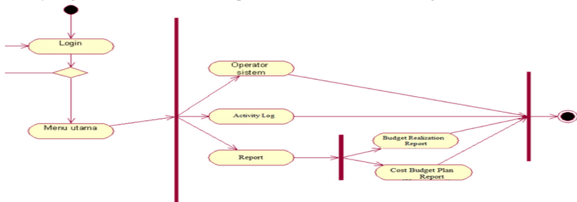
Fig 5. Superadmin main menu activity diagram
