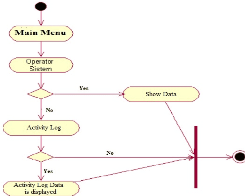
Fig 12. Activity Diagram system operator form and Activity Log
