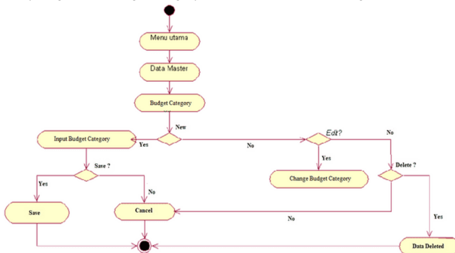
Fig 7. Activity Diagram of budget data
