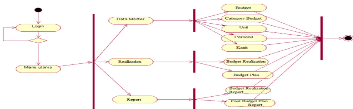
Fig 4. Activity diagram menu utama admin
