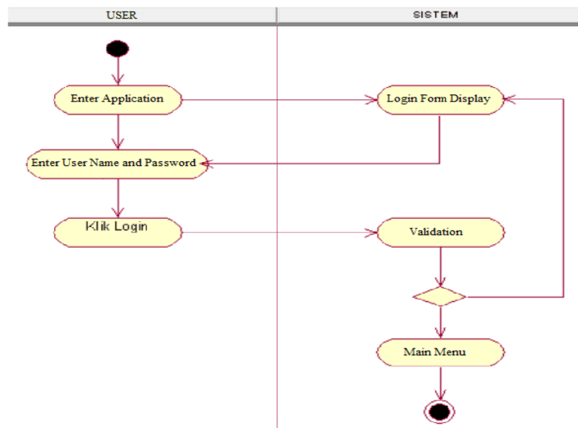
Fig 3. Activity Diagram login
