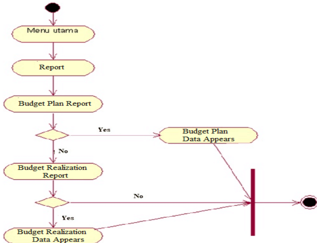
Fig 13. ctivity Diagram form laporan
