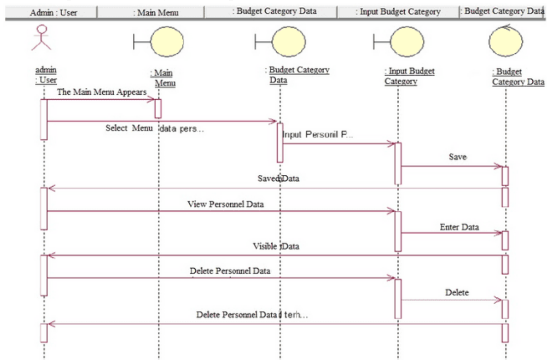
Fig 15. Sequence diagram form personnel data
