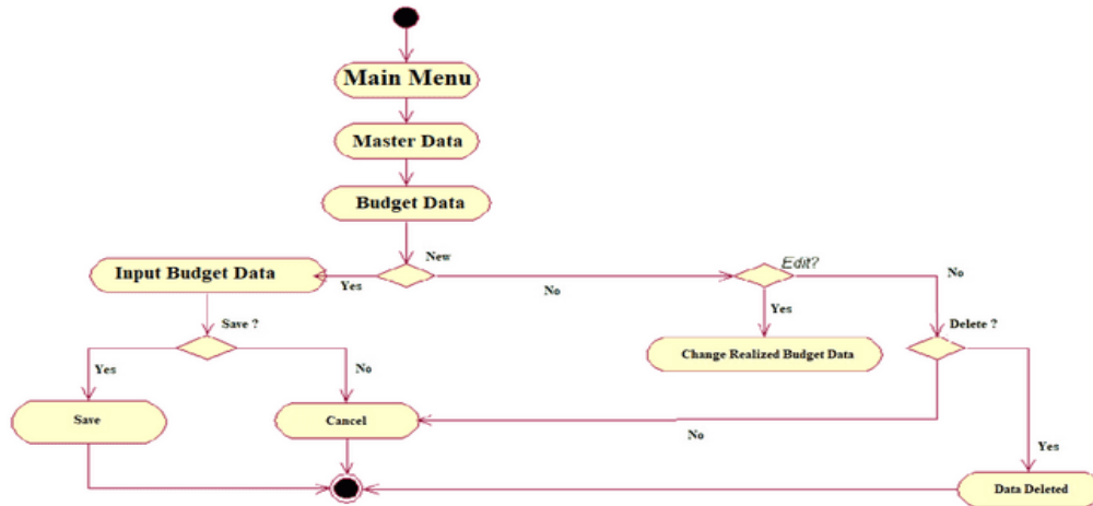
Fig 6. Activity diagram menu budget data
