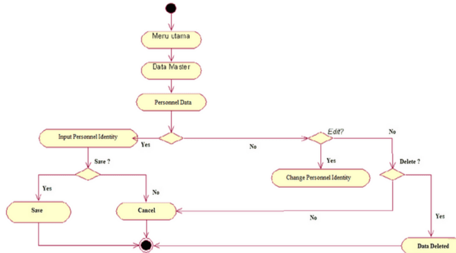
Fig 9. Activity diagram menu data personil
