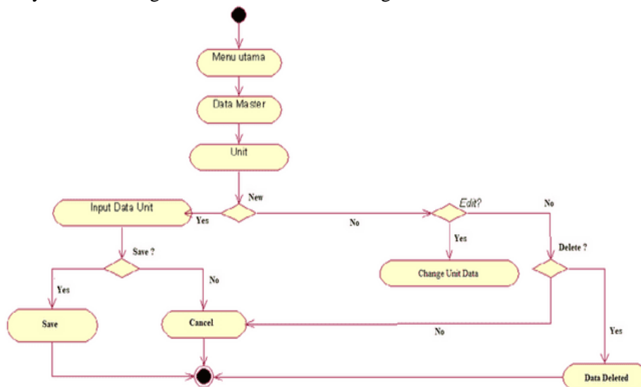
Fig 8. Activity Diagram data unit
