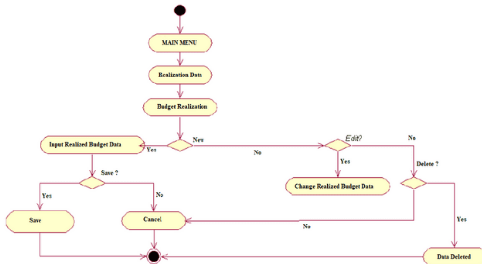
Fig 10. Activity Diagram form for budget realization
