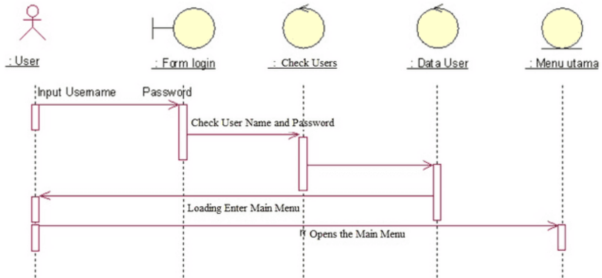
Fig 14. Sequence diagram logged into the system
