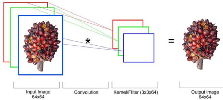
Fig 3. Convolution Process
