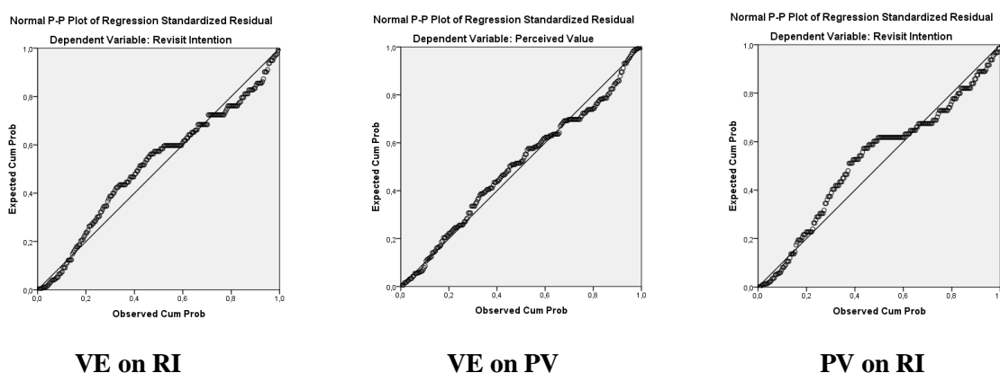
Fig 2. Output Normal Probability Plot SPSS v.24
