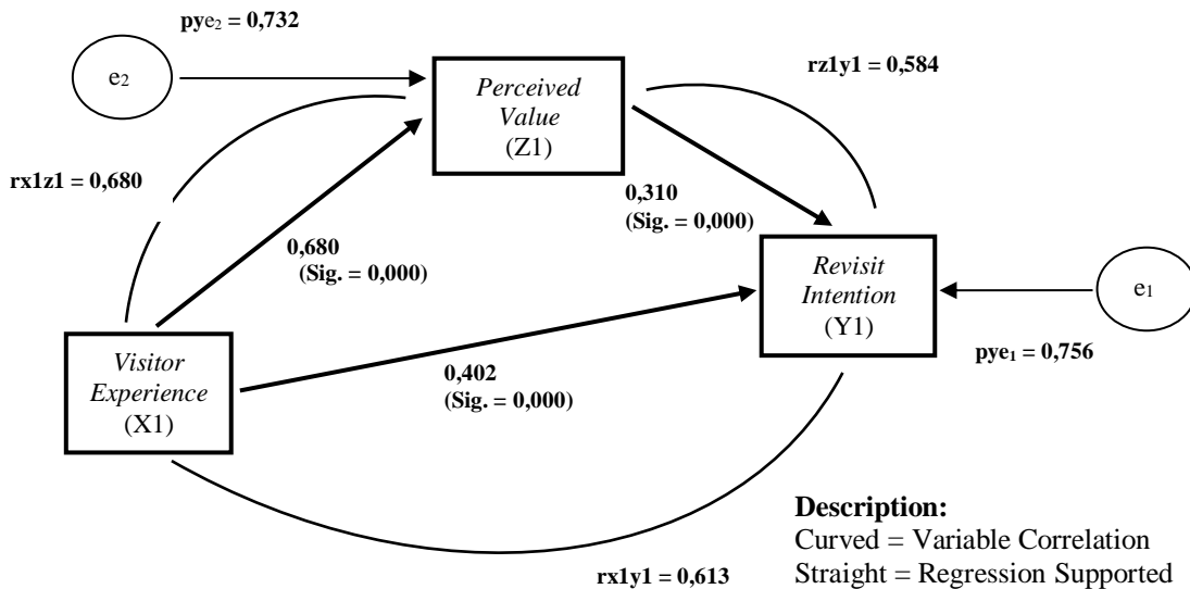
Fig 3. Results of Path and Correlation Analysis Model
